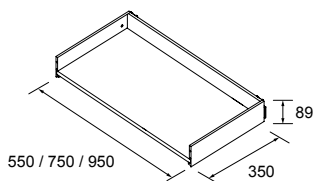
METALLIC DRAWER WITHOUT PIPE CUTOUT
