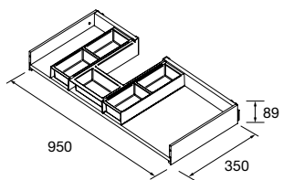
METALLIC DRAWER WITH PIPE CUTOUT, RIGHT
