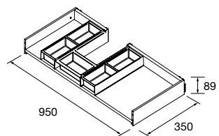
METALLIC DRAWER WITH PIPE CUTOUT, RIGHT
