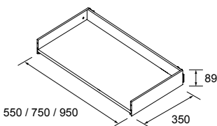
METALLIC DRAWER WITHOUT PIPE CUTOUT
