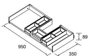
METALLIC DRAWER WITH PIPE CUTOUT, LEFT
