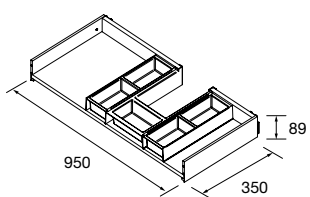
METALLIC DRAWER WITH PIPE CUTOUT, LEFT
