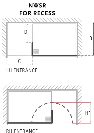
RH Entrance Hinged Return
