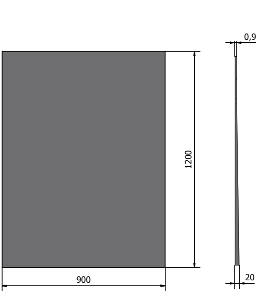
XPS Sloping Board 20mm For Timber or Concrete Floors
