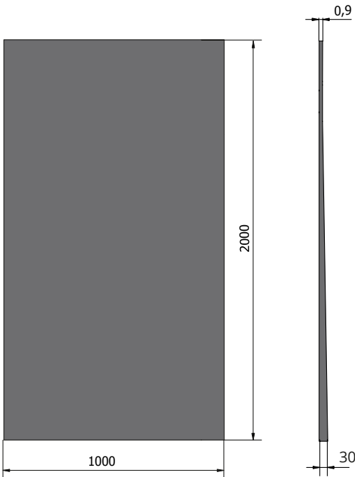
XPS Sloping Board 30mm (2 pieces) For Timber or Concrete Floors
