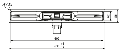
PRO 72 Linear Drain 600mm
