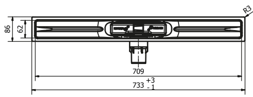
PRO 72 Linear Drain 700mm
