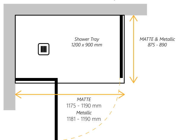
Adjustment range for enclosures (1200 x 900 mm used as example)
