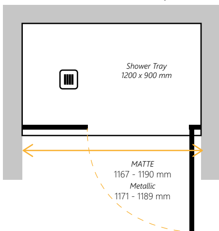
Adjustment range in a recess (1200 mm used as example)
